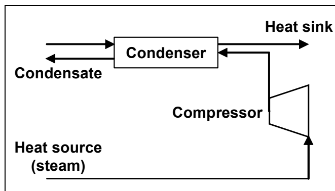
Figure 3.10: Simple MVR installation [18, Åsbland, 2005]
