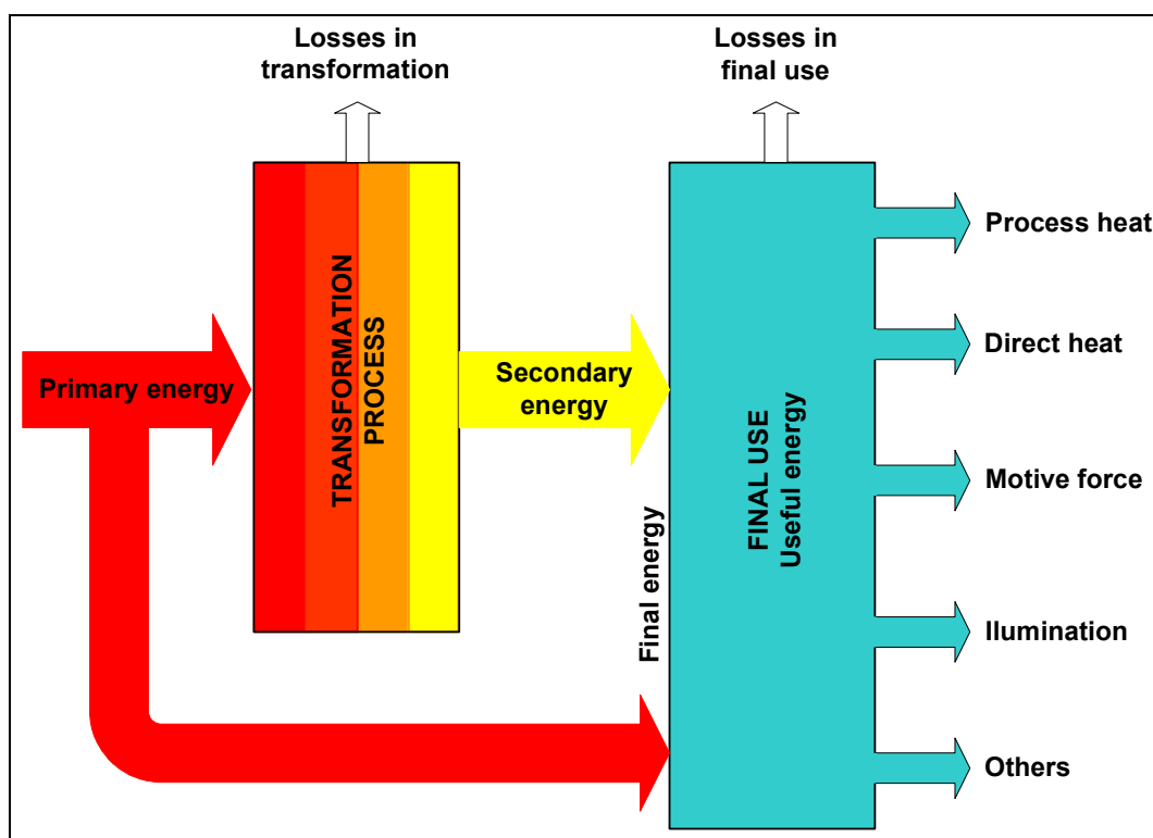
Figure 1.6: Definition of primary, secondary and final energies [260, TWG, 2008]
