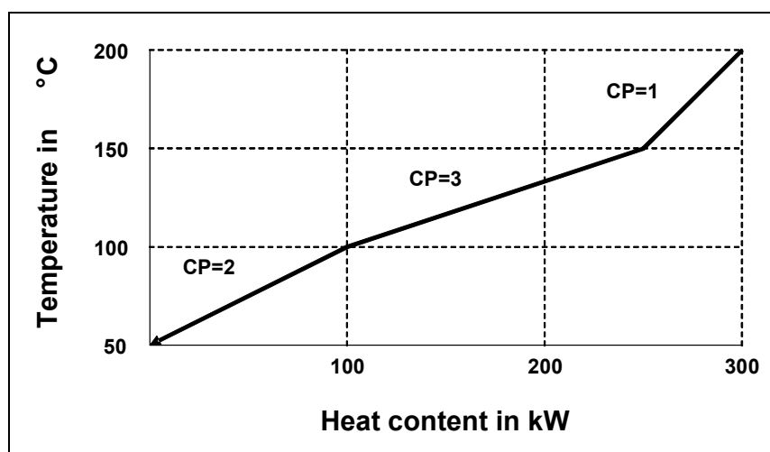
Figure 2.12: Hot composite curve
