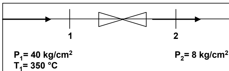
Figure 7.2: Steam throttling process
