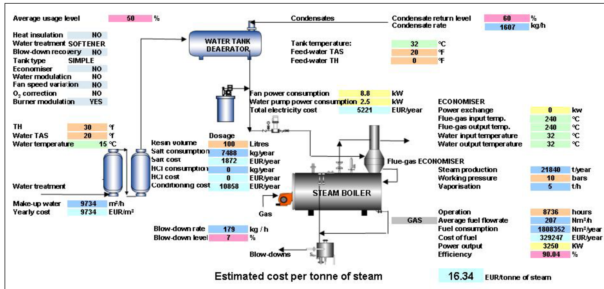
Figure 3.6: Modern control system optimising boiler usage
