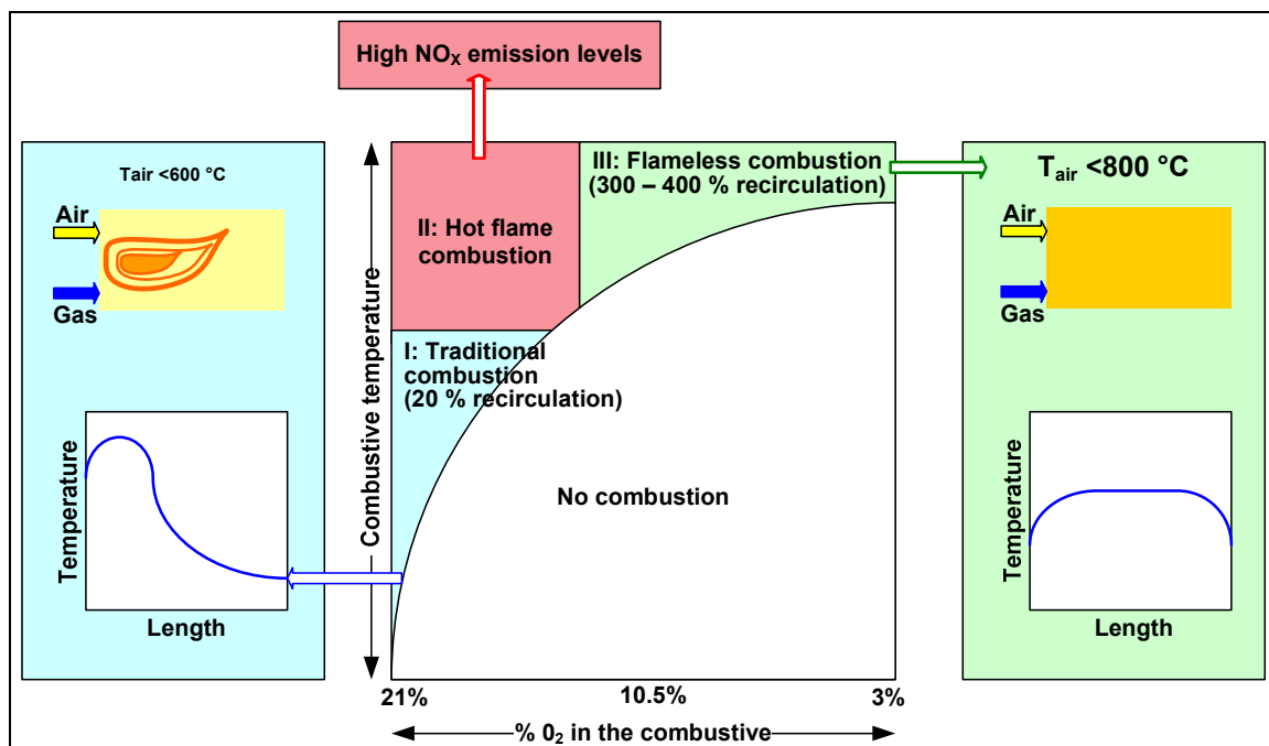
Figure 5.3: Flameless combustion conditions
