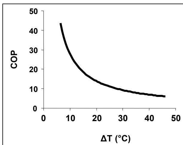
Figure 3.11: COP versus temperature lift for a typical MVR system [18, Åsbland, 2005]
