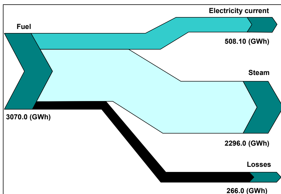
Figure 2.7: Sankey diagram: fuel and losses in a typical factory [186, UBA_AT]
