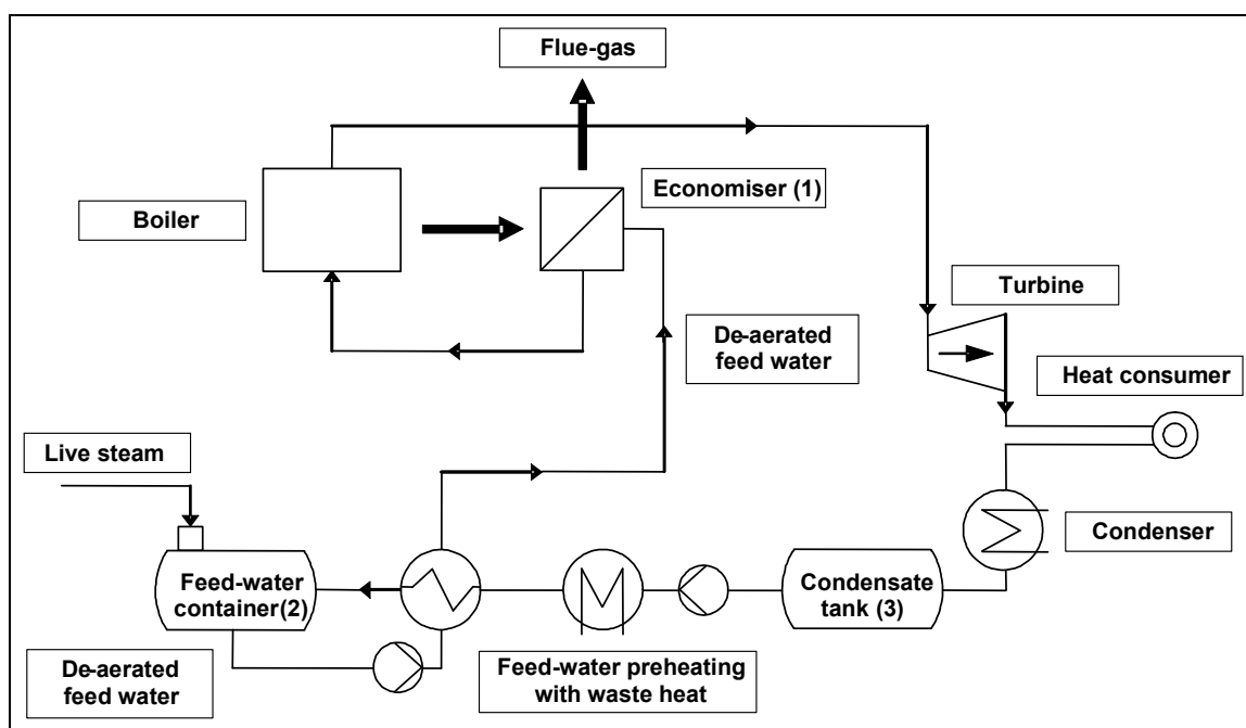
Figure 3.7: Feed-water preheating [28, Berger, 2005]
